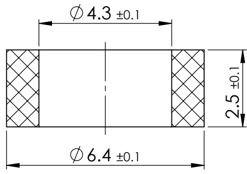
SECTION X-X
